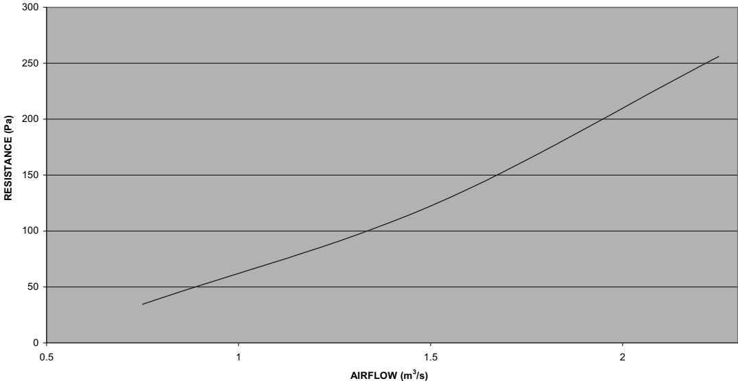
RESISTANCE AGAINST AIR FLOW UVC 4500
